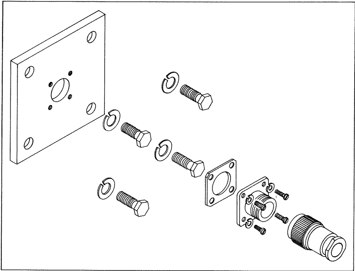
Typical Assembly
