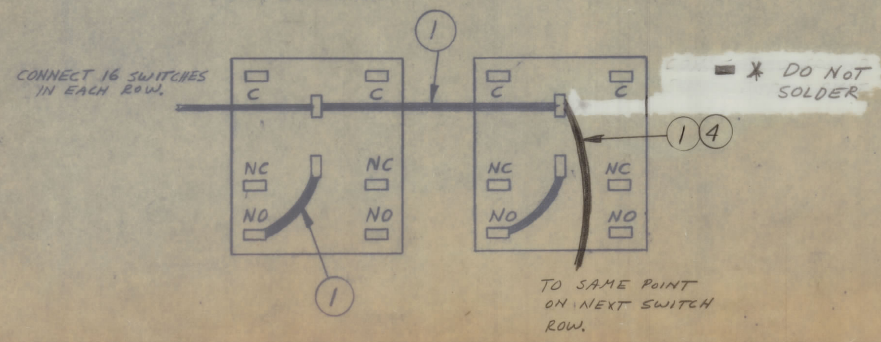
TYPICAL STEP 2 ALL SWITCHES
