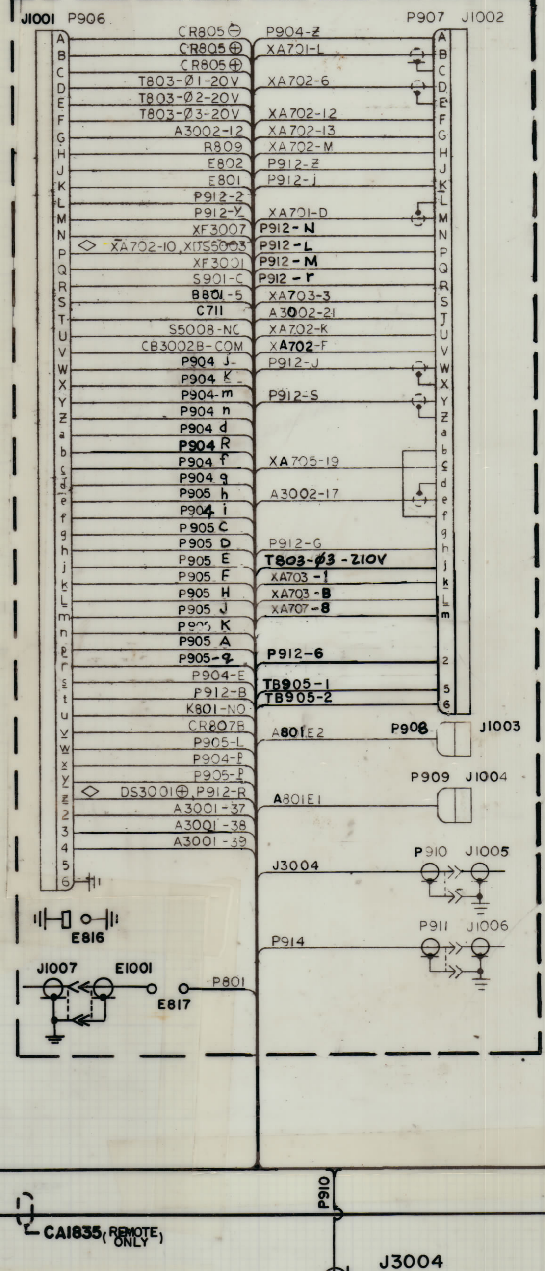
DRIVER DRAWER (AX5232) REF CK2179
