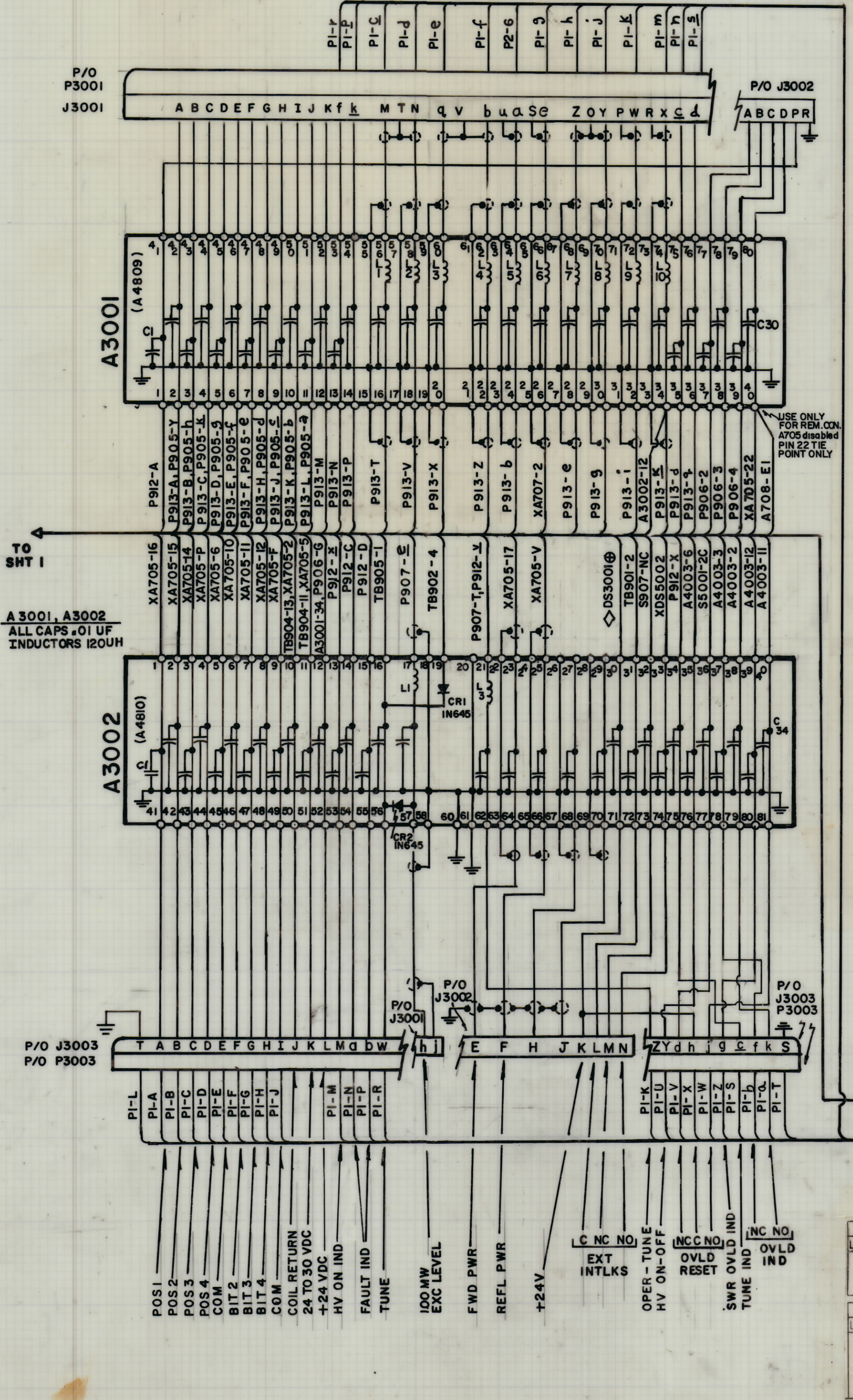
DRIVER DRAWER (AX5232) REF CK2179
