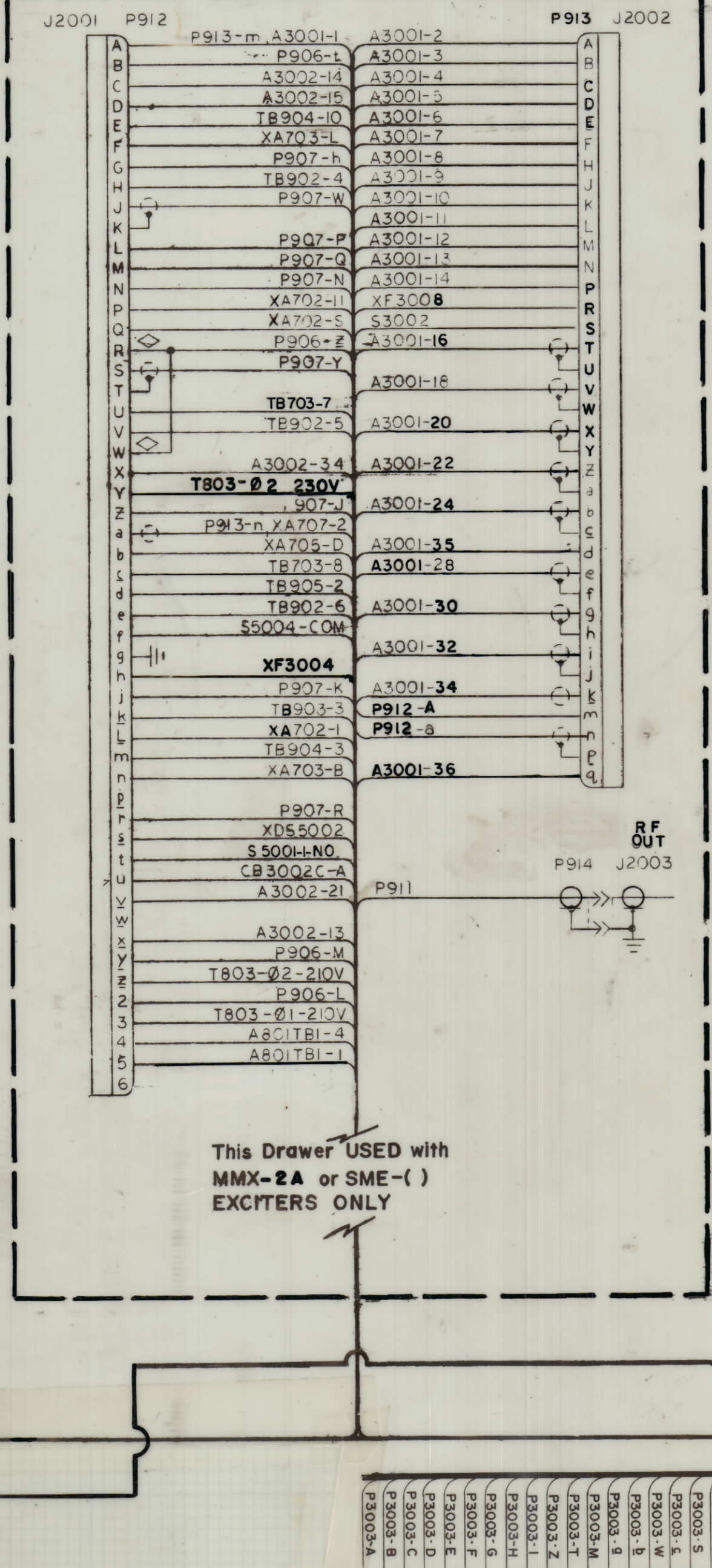
REFERENCE CK1955 EXCITER DRAWER FOR MMX-2A (AX5168)
