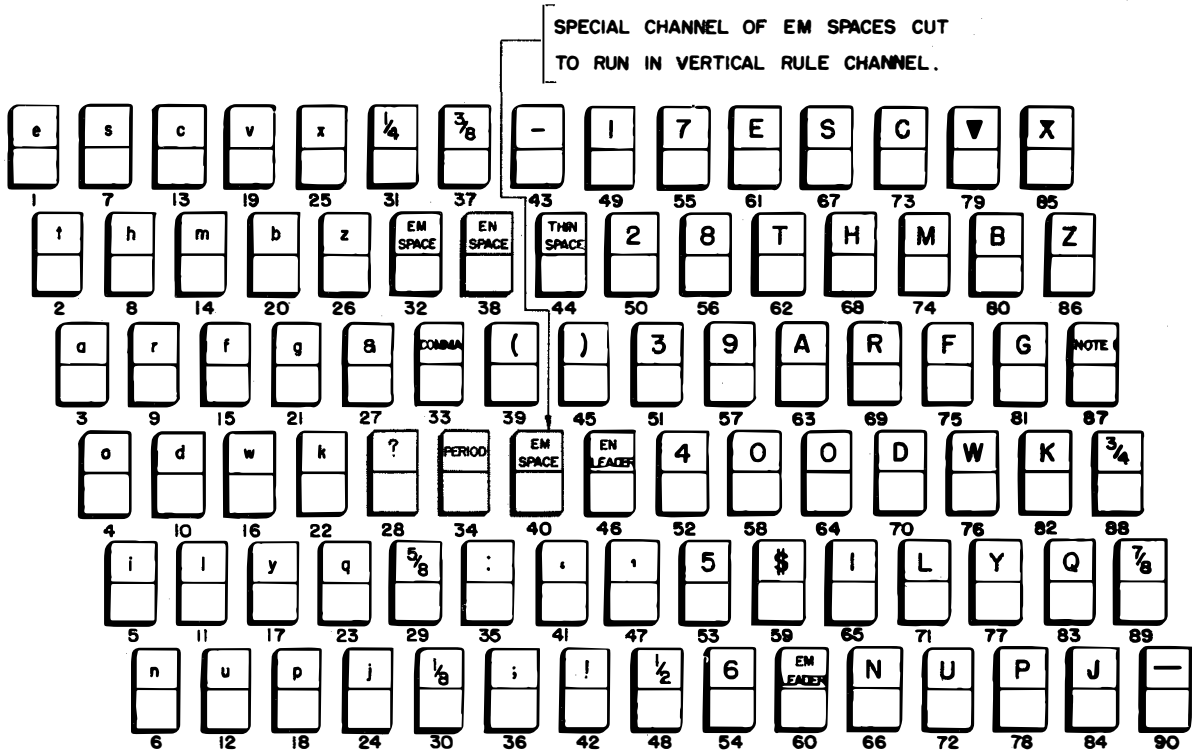
STANDARD LAYOUT SUPPLIED FOR TELETYPESETTER OPERATION WHERE FRACTIONS ARE REQUIRED
