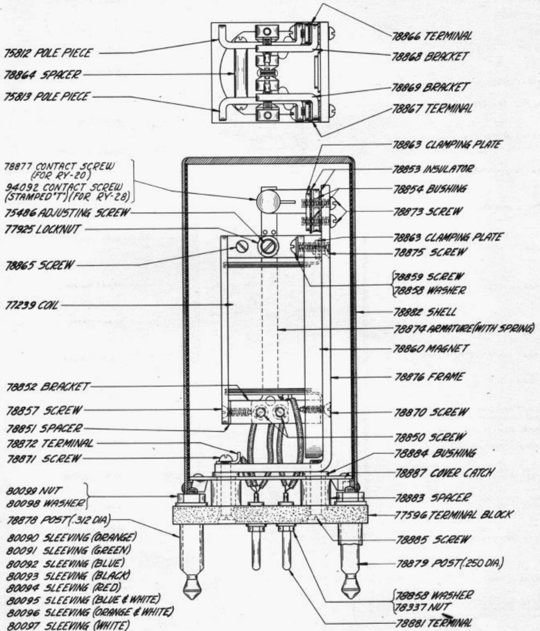
RY-20 LINE RELAY (W.E.CO 215-A) RY-28 LINE RELAY (W.E.CO 215-H)
