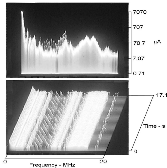
Figure 21 EMI Current Flowing on PDU Power Conductor
