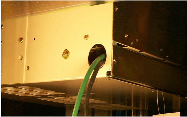
Figure 50 Unfiltered Conductors Exiting a Switching Power Supply
