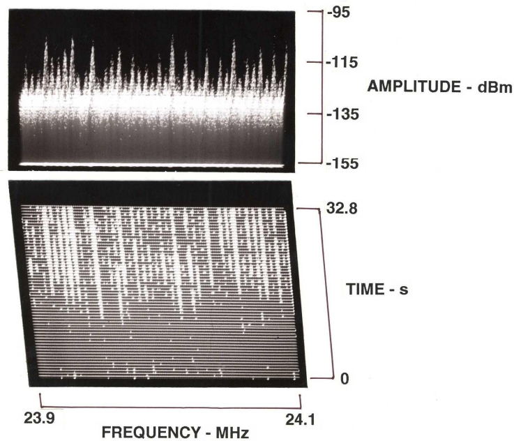
Figure 8 Above-Band IM Products
