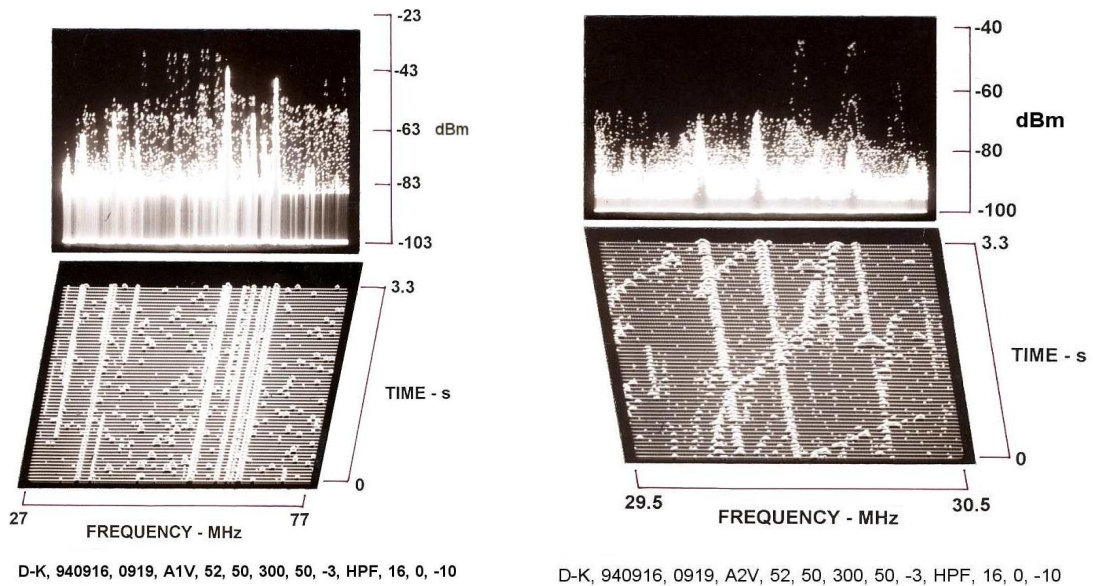
Figure 32 Intermittent Interference from Frequency-Hopping and ISM Emissions
