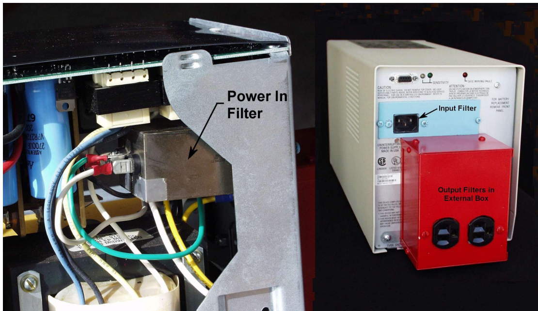
Figure 46 UPS Modified to Comply with BFG Principles
