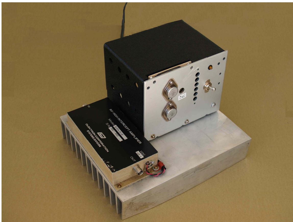
Figure 61 Example of a Preamplifier for the HF Band
