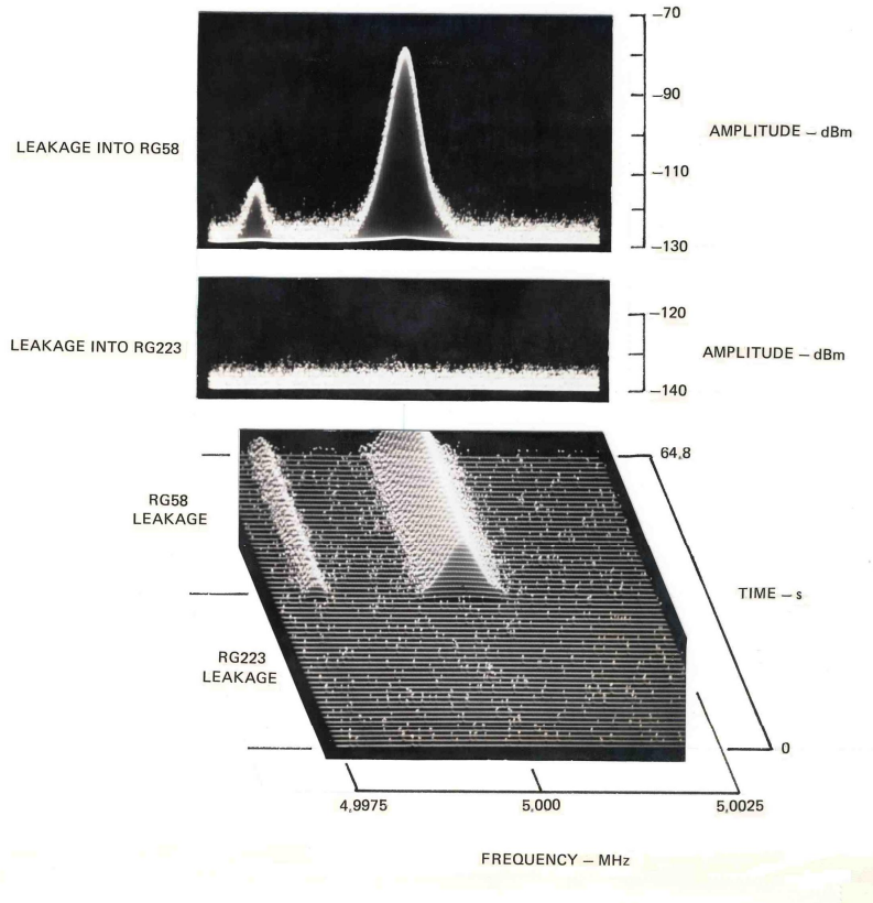
Figure 10 Example of Leakage into Coaxial Cables
