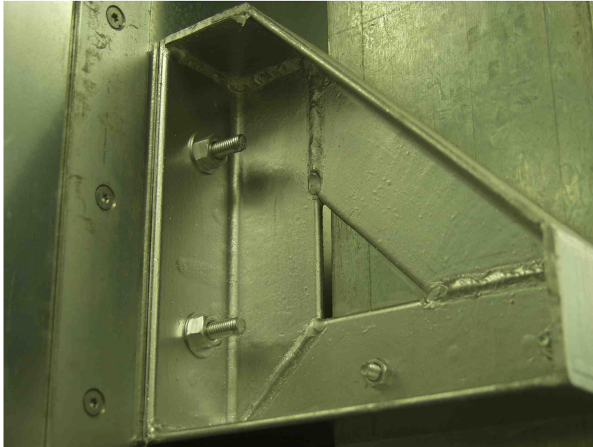
Figure 25 Weld on Galvanized Steel inside a Radio-Receiving Building
