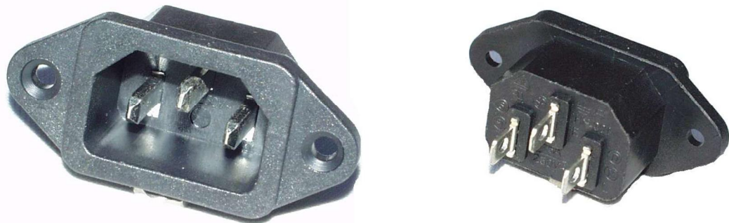
Figure 42 Chassis Power Connector that does not comply with BFG Needs
