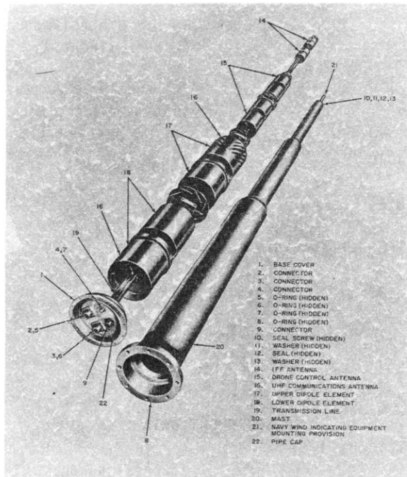
ANTENNA AS-1390/U
