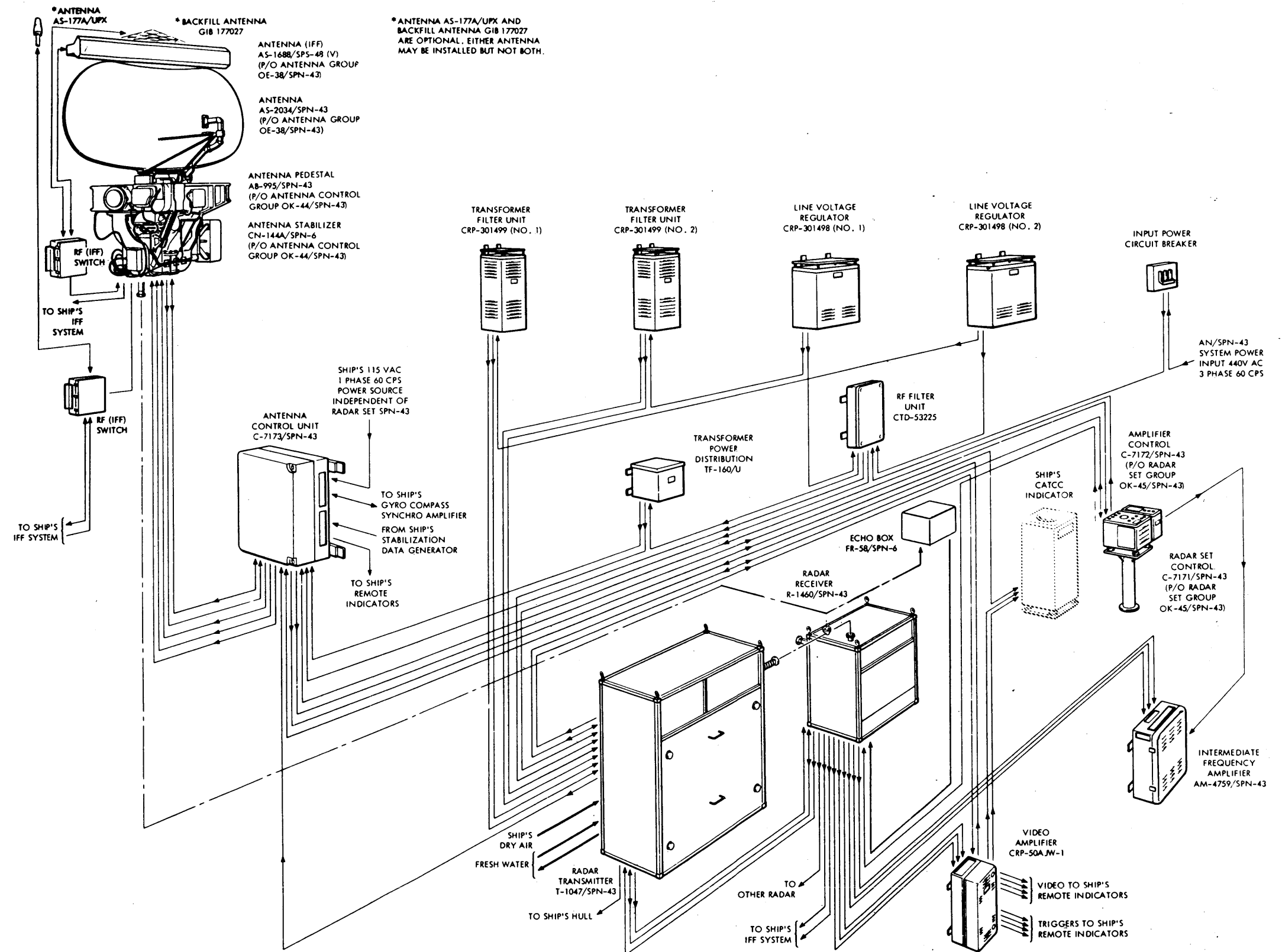
Figure 7-19.—Radar Set AN/SPN-43.
