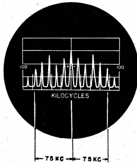
Figure 25. Frequency Deviation of \pm 75\text{KC} at a Modulation Frequency of 15KC
