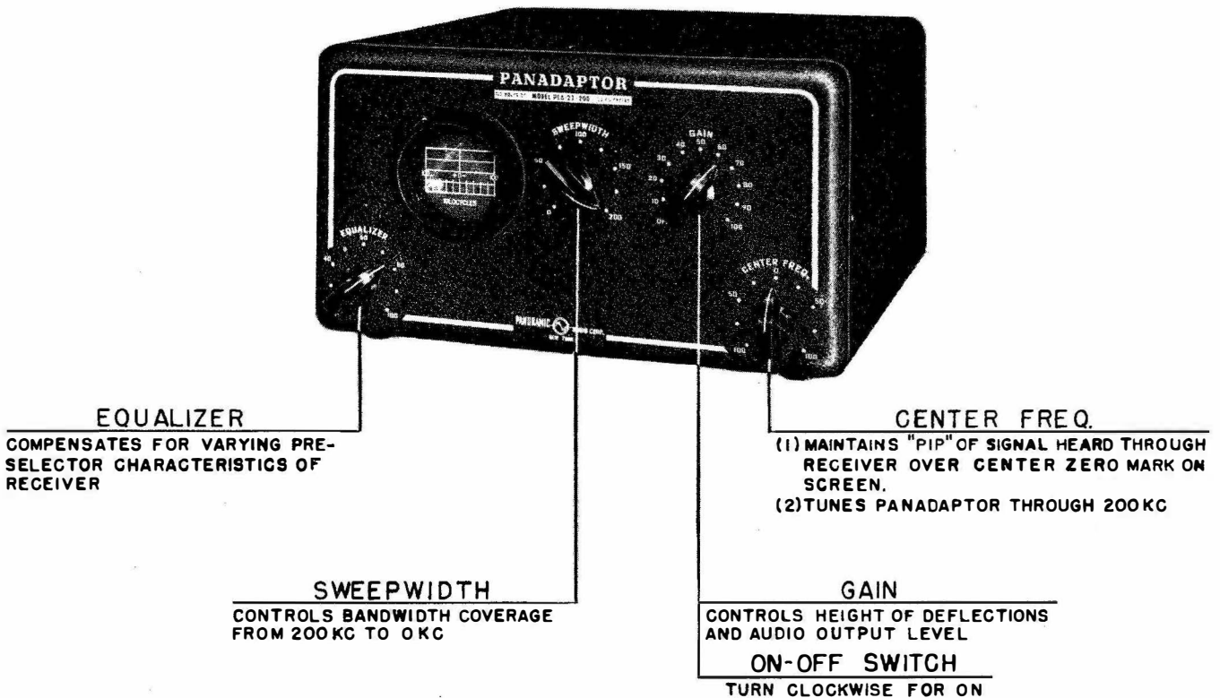
Figure 3. Main Operating Controls
