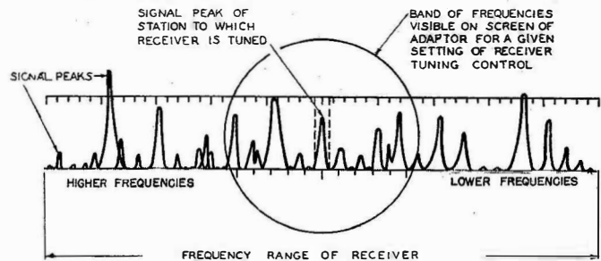
Figure 1. Portion of the Radio Frequency Spectrum
