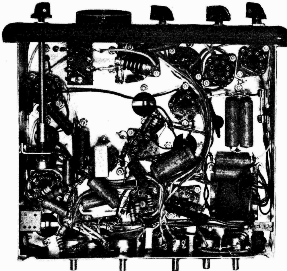
Figure 35. Bottom View of Chassis
